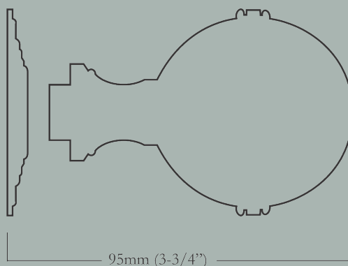
Overall Projection
