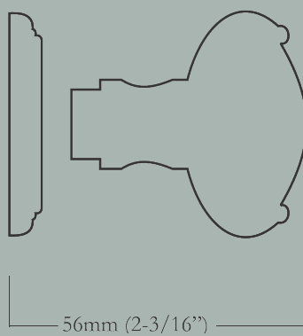
Overall Projection
