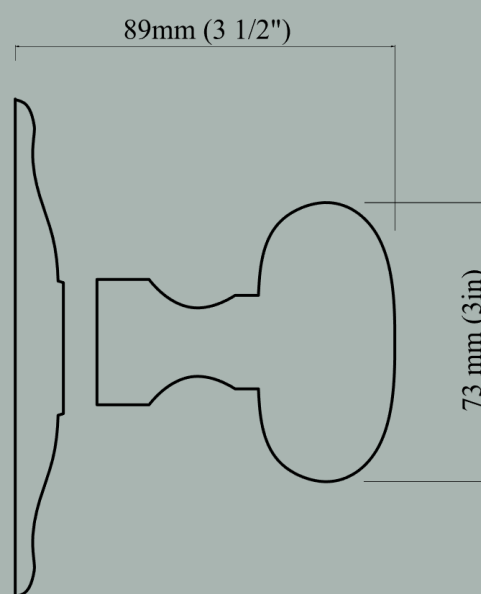
OverAll Projection
