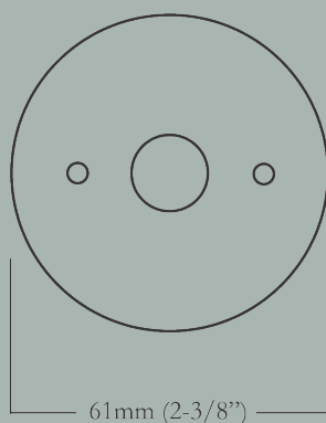
Escutcheon Diameter
