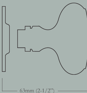
Overall Projection
