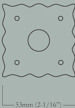
Escutcheon Diameter
