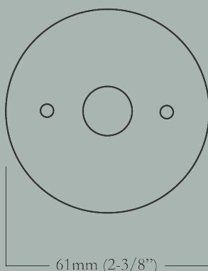
Escutcheon Diameter
