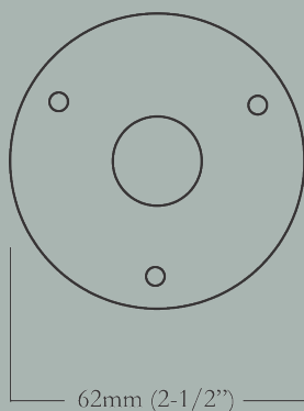
Escutcheon Diameter
