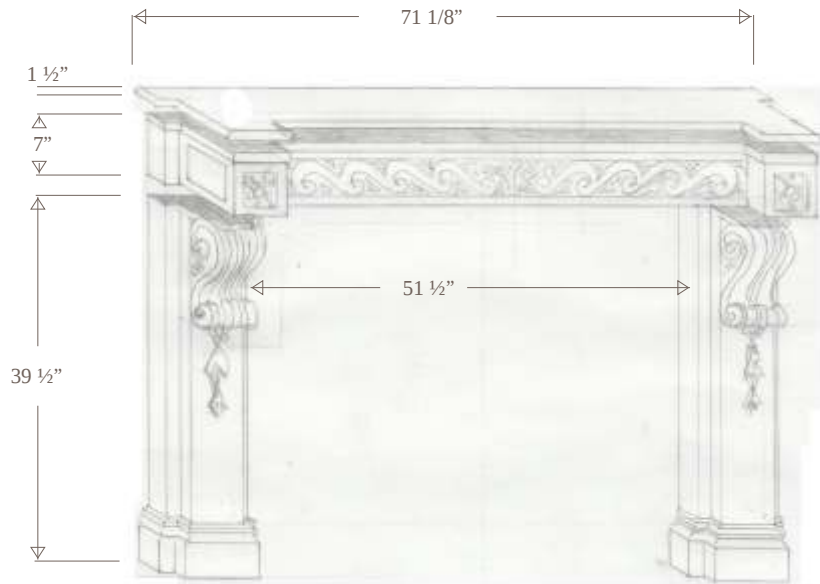
Isometric
