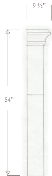
Side Elevation
