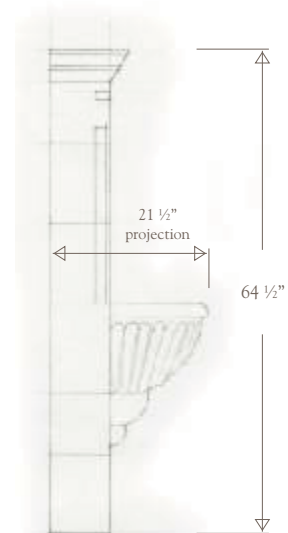
Side Elevation
