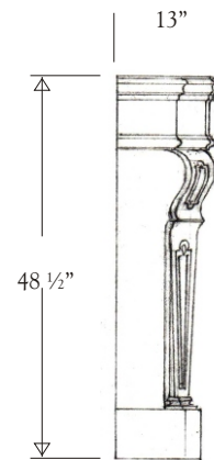
Side Elevation
