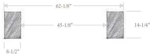
Footprint
